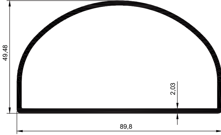
16713 1,304 Kg/Mt
