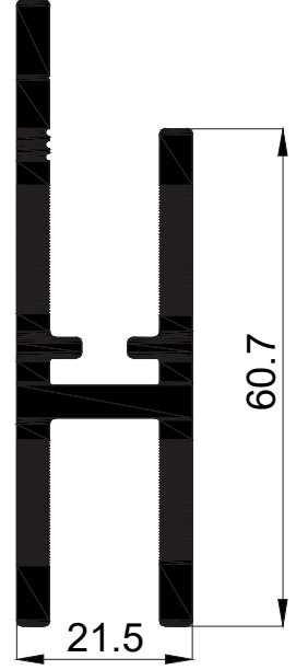
16712 1,671 Kg/Mt
