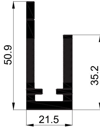
16709 1,109 Kg/Mt
