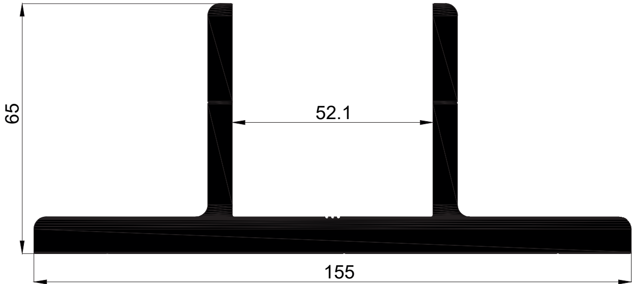
16738 5,881 Kg/Mt
